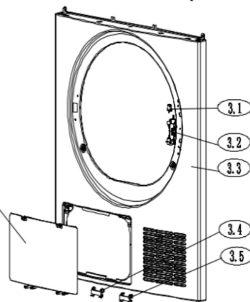
Front Panel Subassembly
