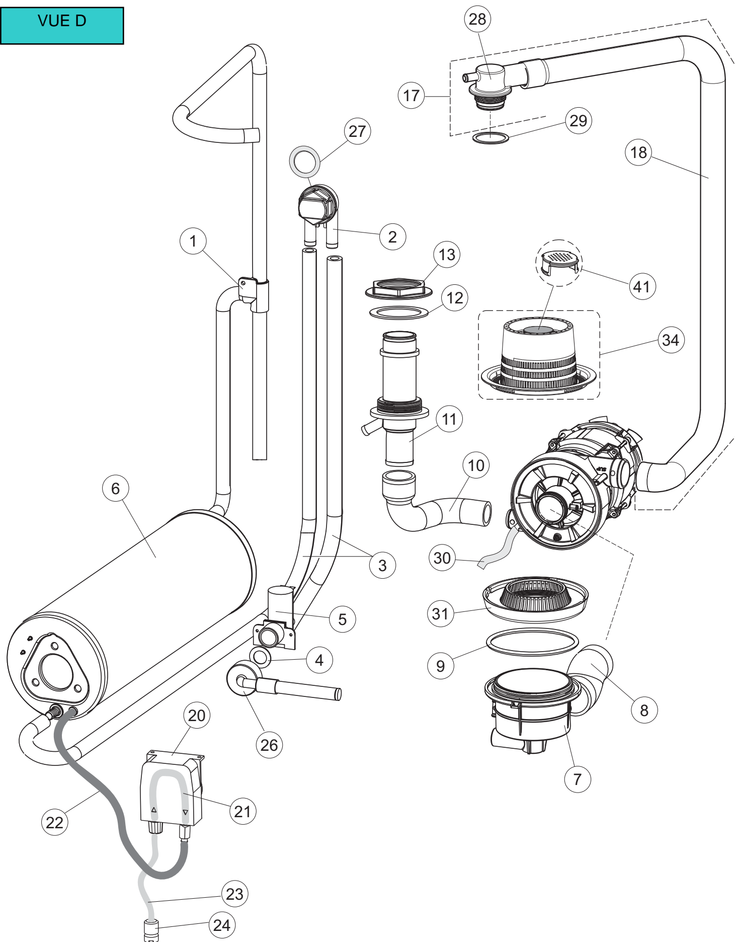
Drain Pump
