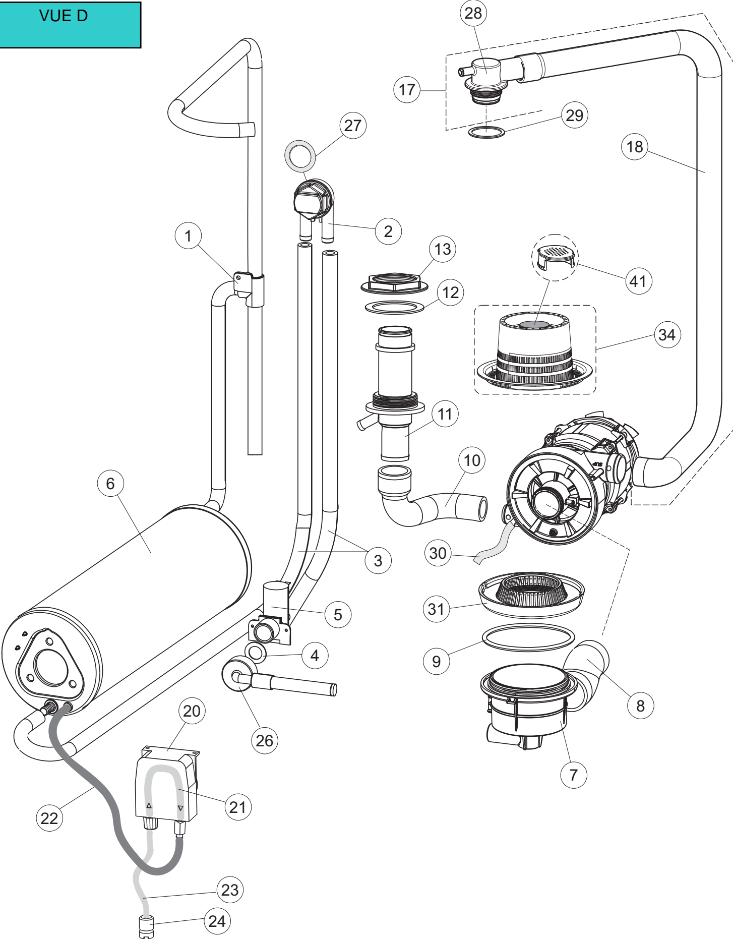
DRAIN PUMP
