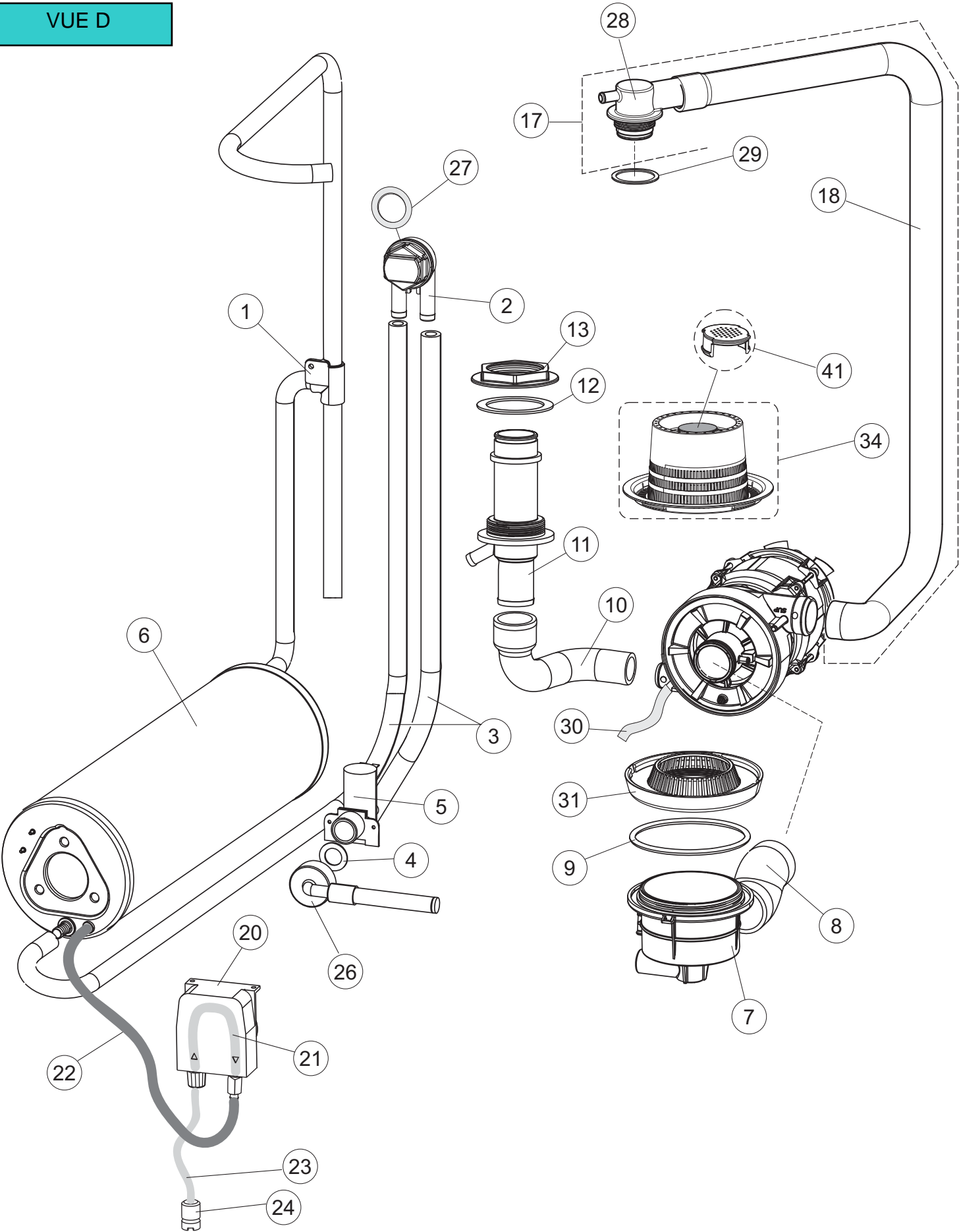
DRAIN PUMP
