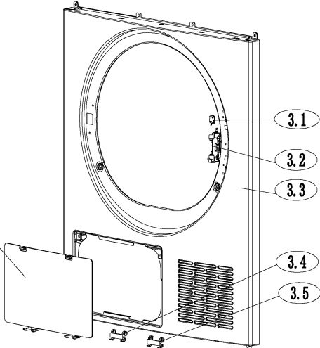
Front Panel Subassembly
