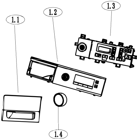
Control Panel Subassembly
