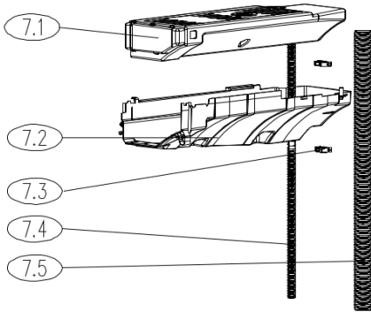
Drawer Subassembly
