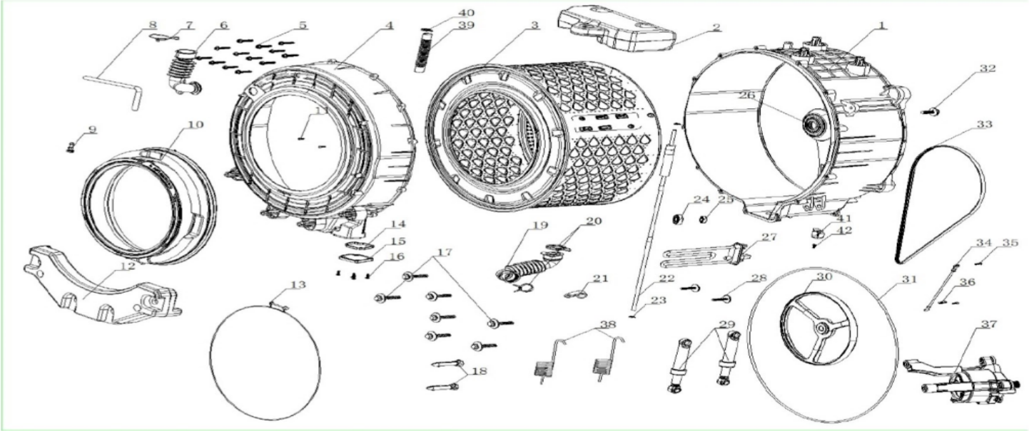
Part 3 Tub assy.
