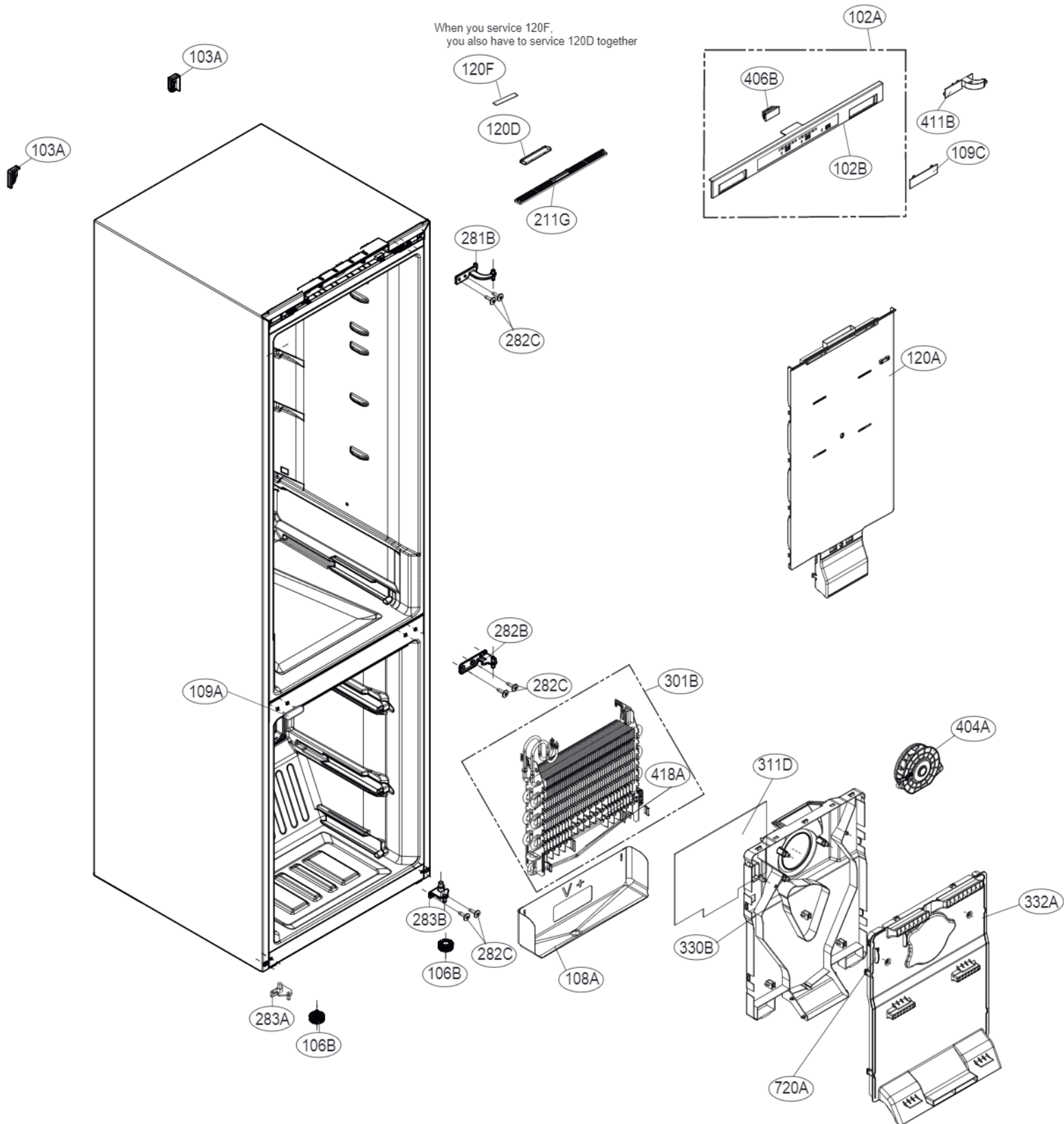
Location 283A includes entire set for reversing doors
