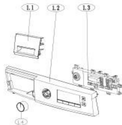
Control Panel Subassembly
