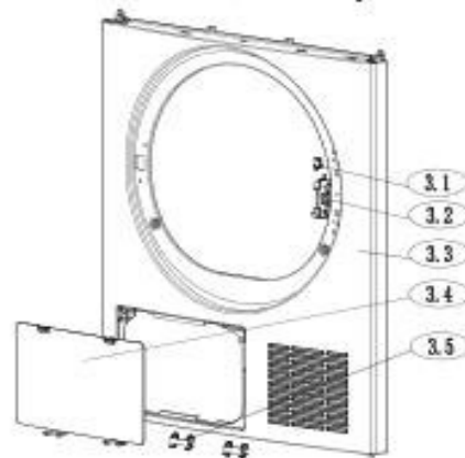
Front Panel Subassembly
