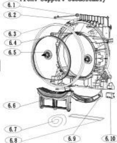
Front Support Subassembly
