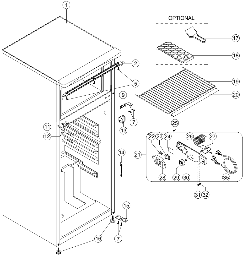
WIRE SHELF DESIGN
