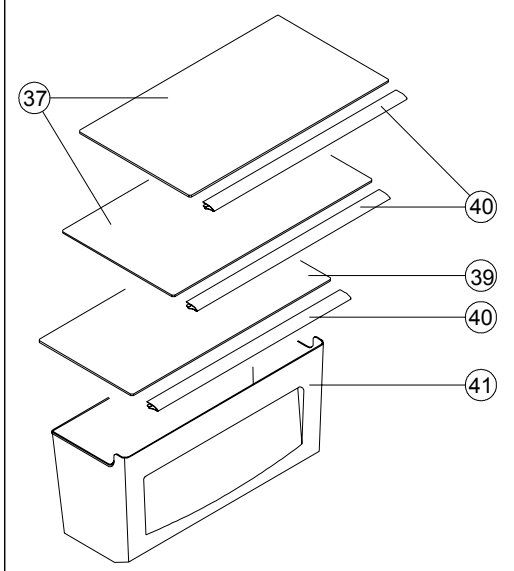
GLASS SHELF DESIGN
