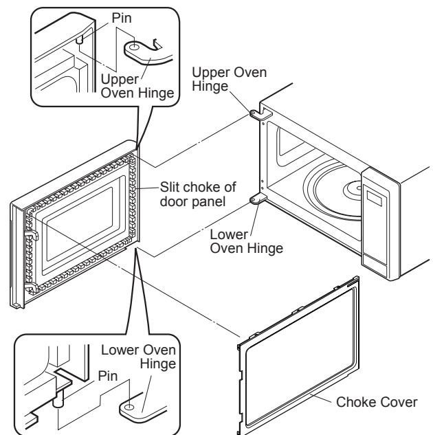
Figure C-8. Door Replacement
