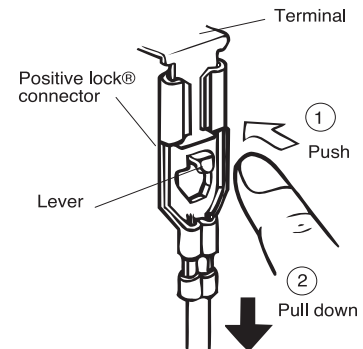
Figure C-2. Positive lock®connector
