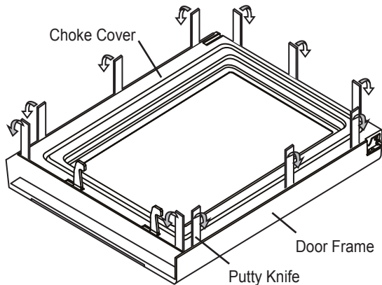
Figure C-7. Door Disassembly
