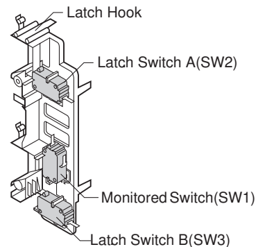
Figure C-5. Switches
