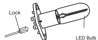
Figure C-3. Oven lamp
