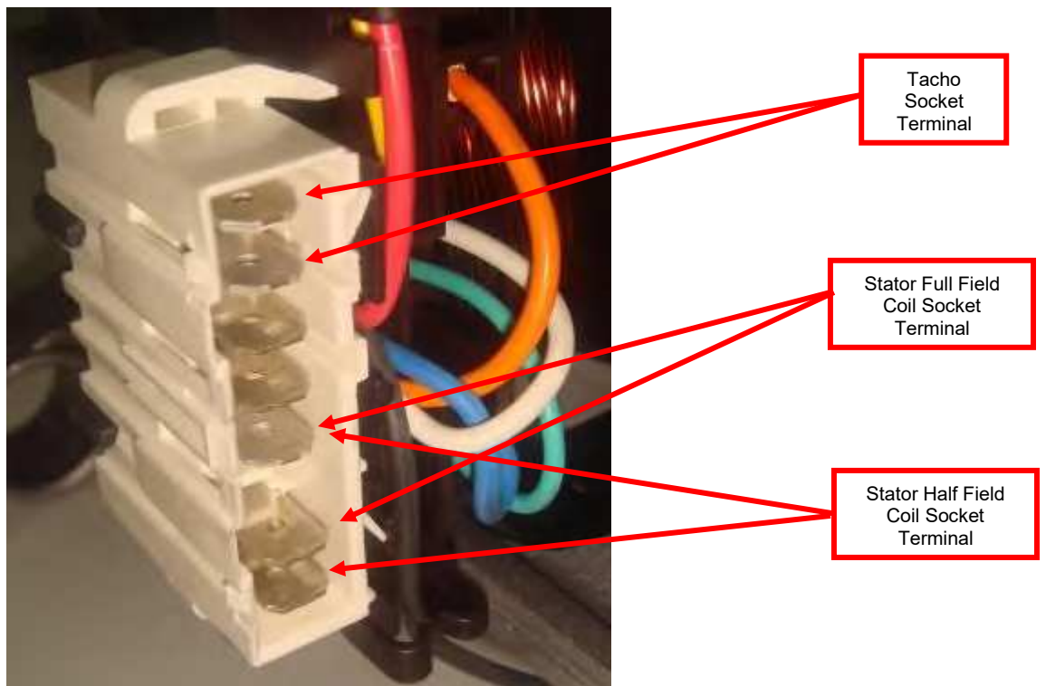
Motor Socket Terminals
