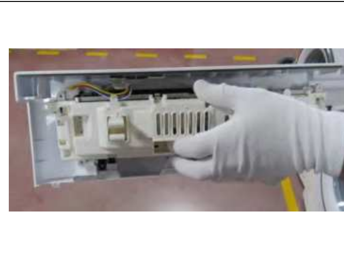
3.2. Push the PCB box and fit to the housing
