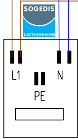
TERMINAL BOX
