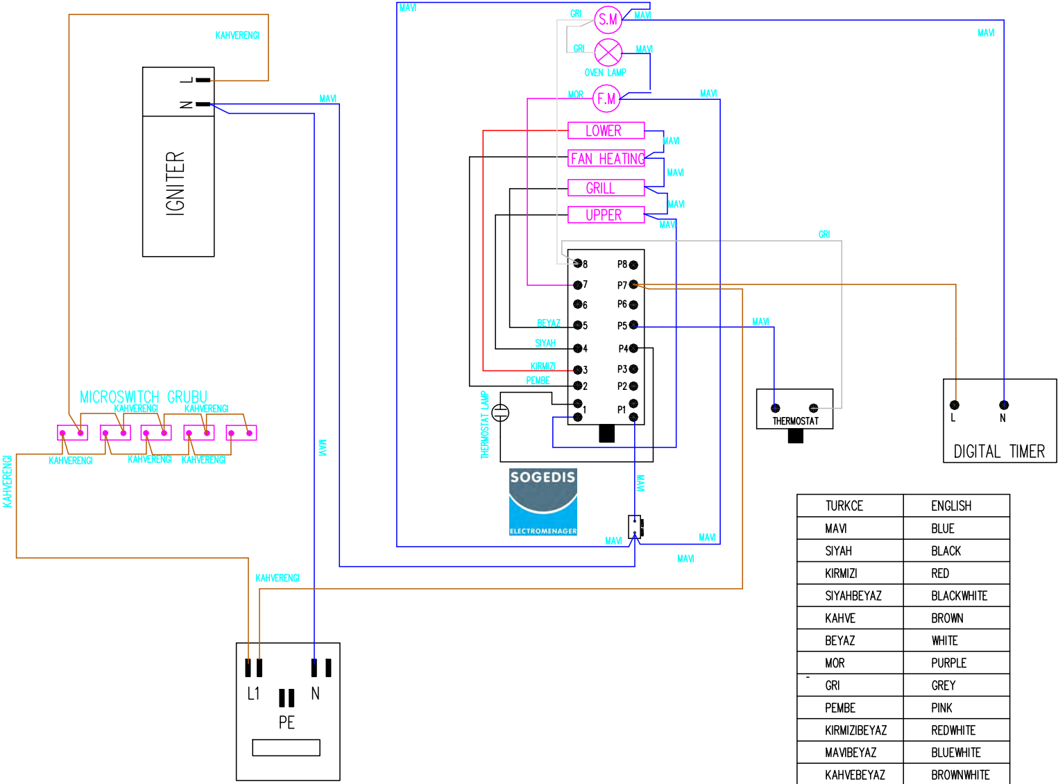
TERMINAL BOX
