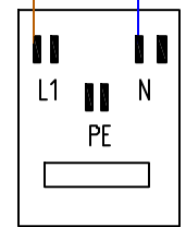
TERMINAL BOX
