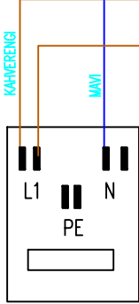
TERMINAL BOX
