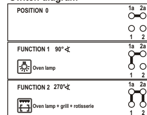
Switch diagram
