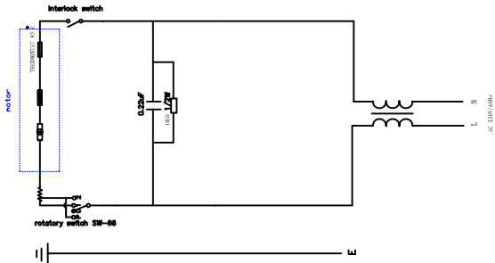
KP-508BG (EK) BLENDER CIRCUIT DIAGRAM
